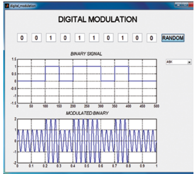
Fig. 4: ASK modulation
